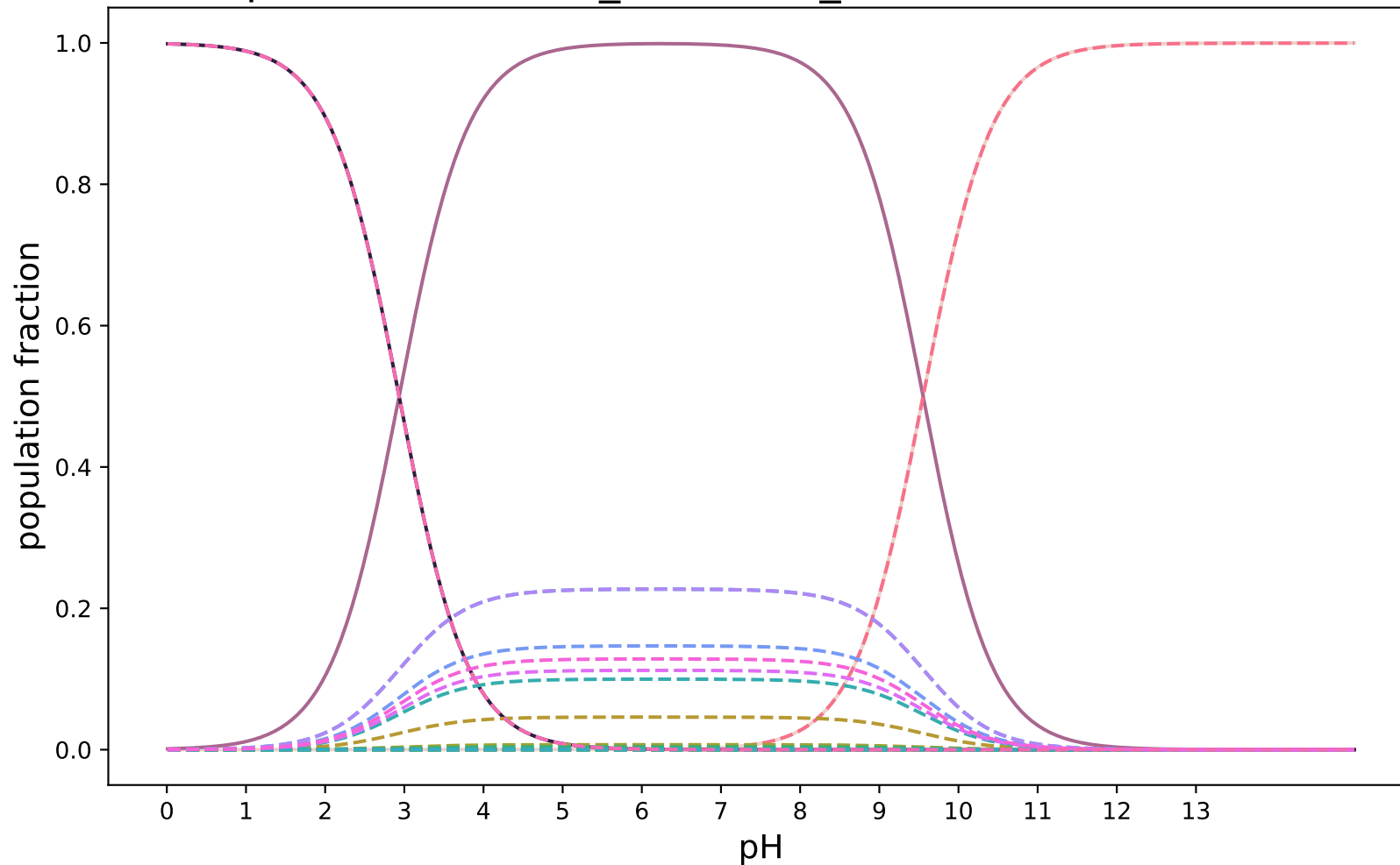
pKa-RobertRaddi_AdaBoost_modified:SAMPL8-21
