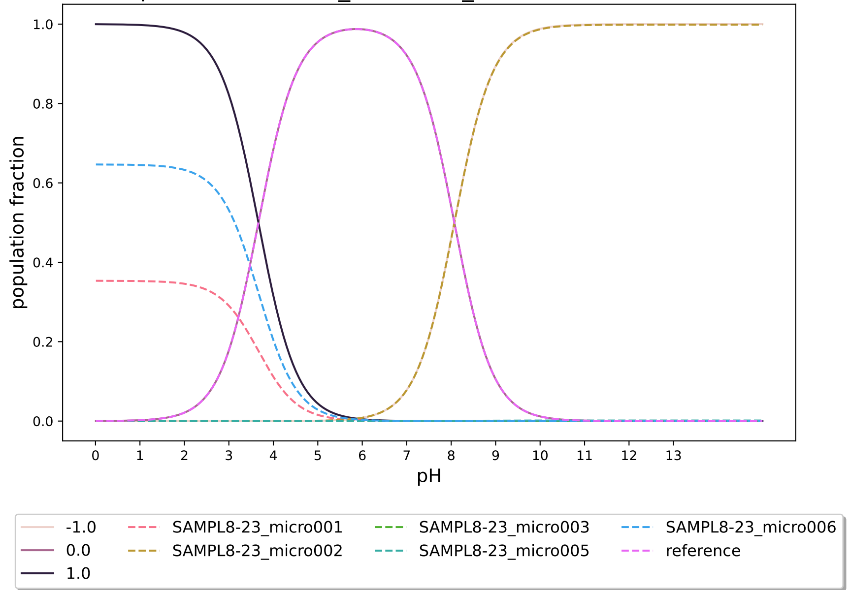
pKa-RobertRaddi_AdaBoost_modified:SAMPL8-23
