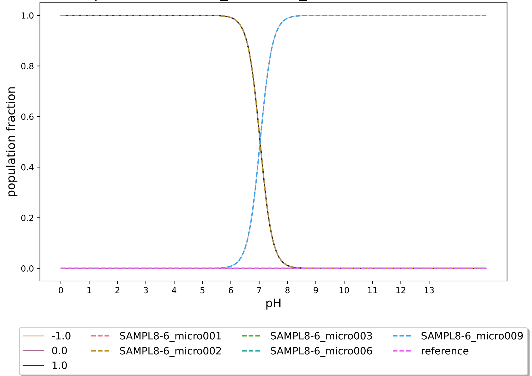
pKa-RobertRaddi_AdaBoost_modified:SAMPL8-6
