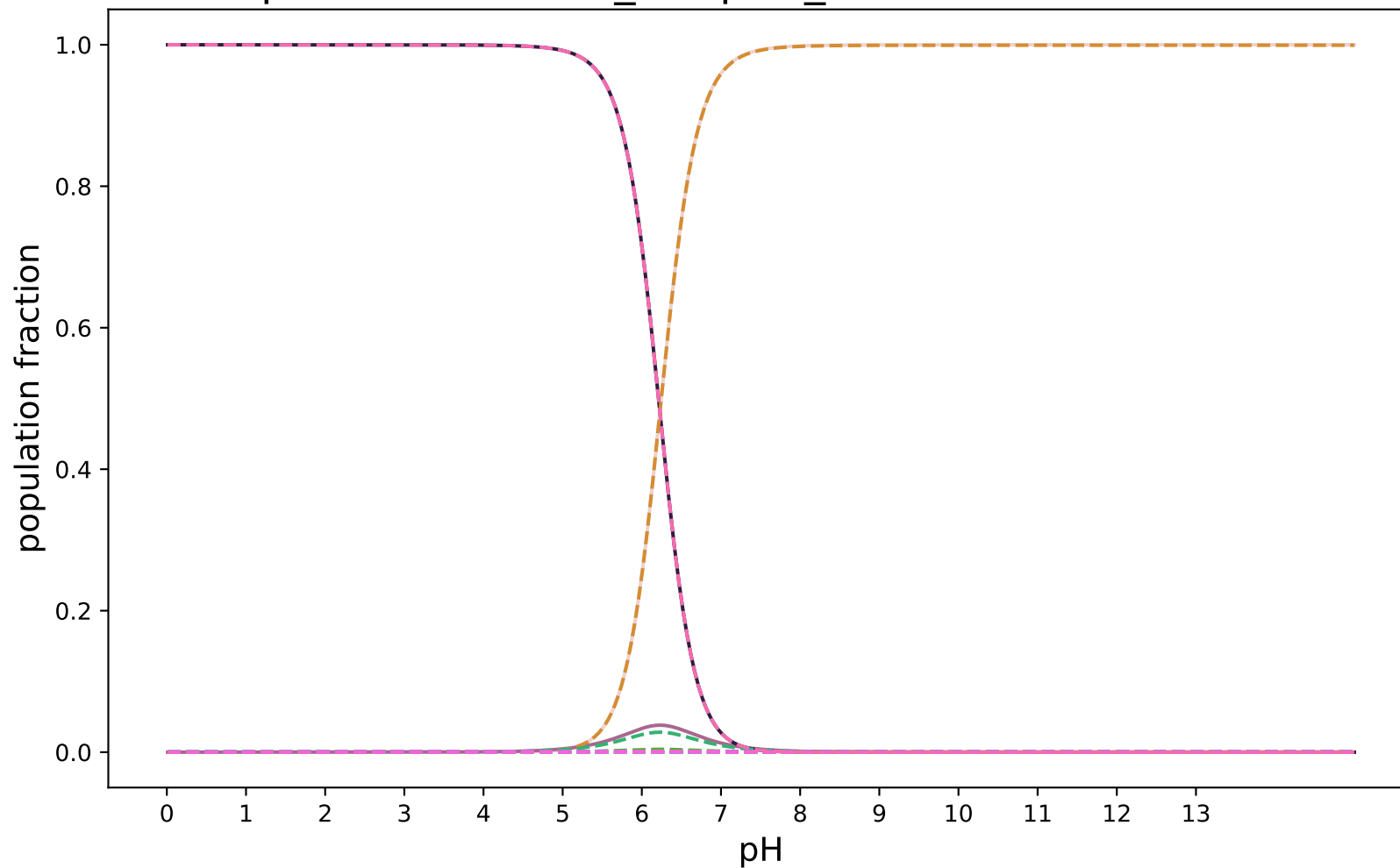
pKa-RobertRaddi_DeepGP_modified:SAMPL8-14
