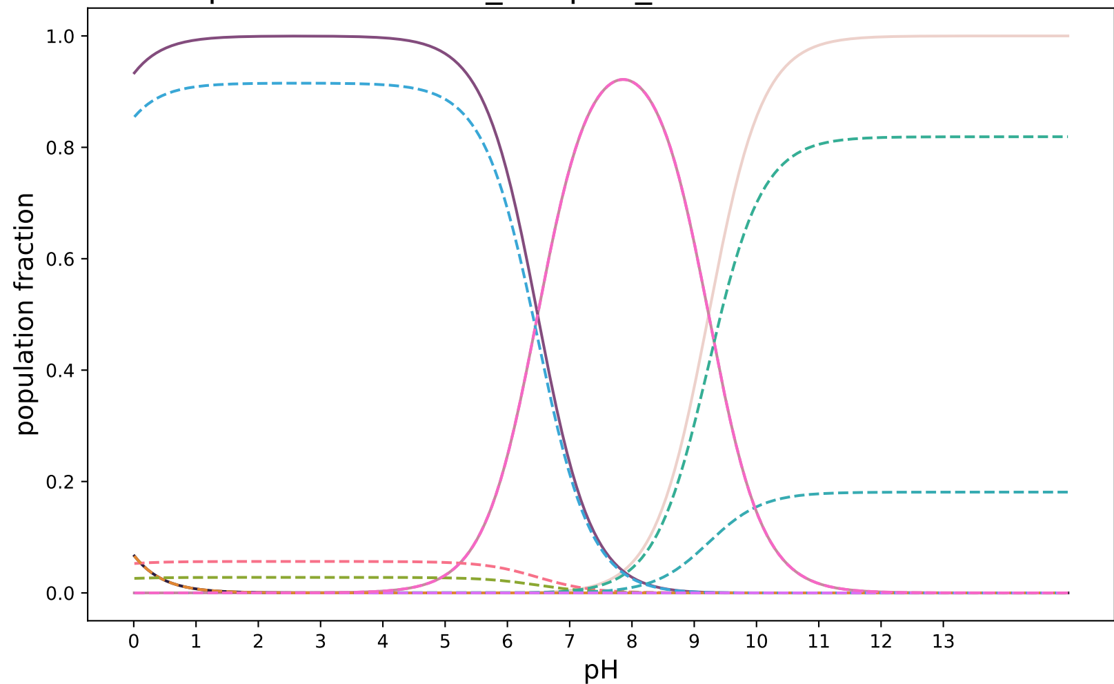
pKa-RobertRaddi_DeepGP_modified:SAMPL8-19
