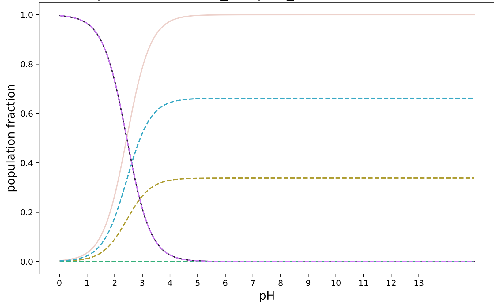
pKa-RobertRaddi_DeepGP_modified:SAMPL8-4
