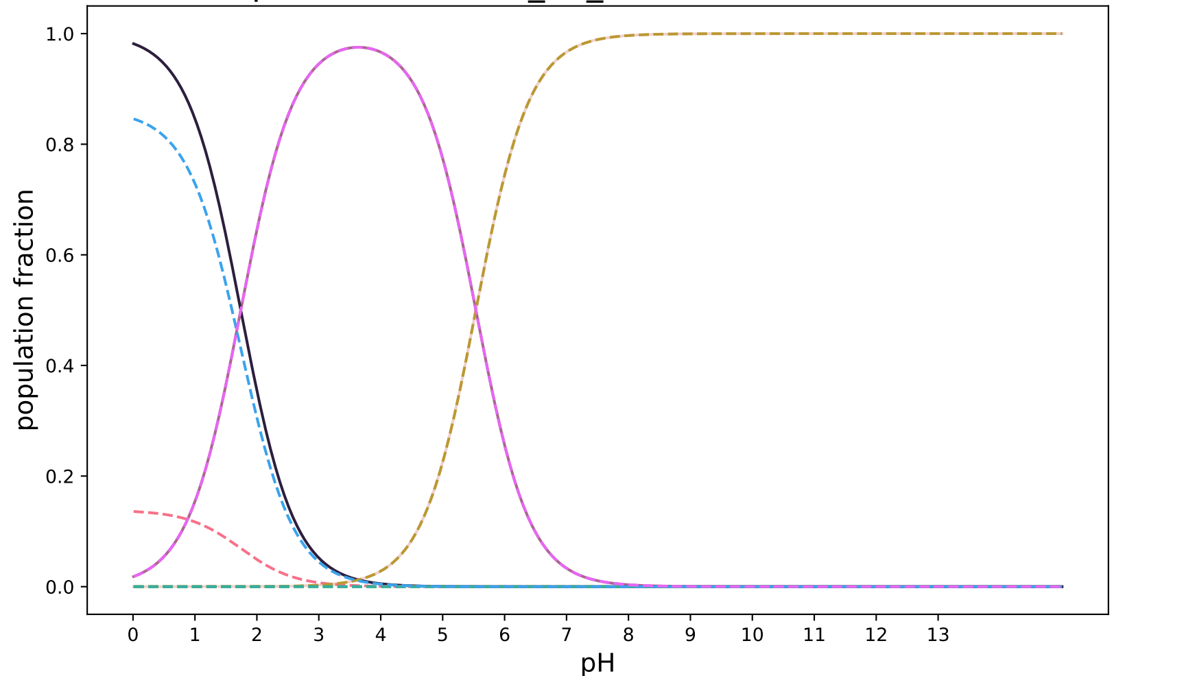
pKa-RobertRaddi_RF_modified:SAMPL8-23
