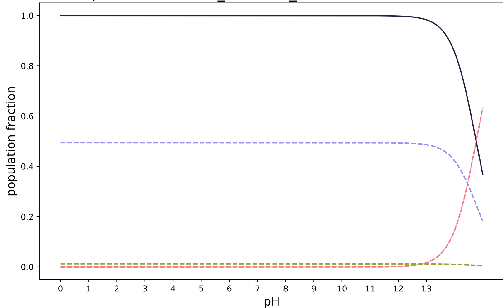
pKa-RobertRaddi_XGBoost_modified:SAMPL8-12
