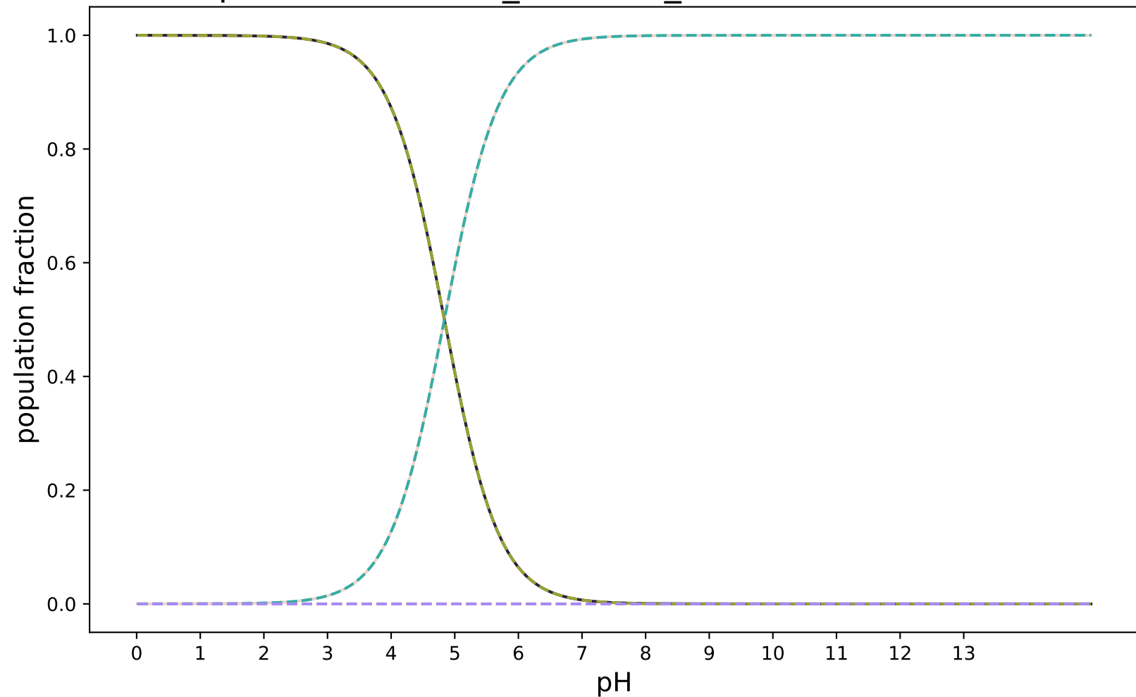
pKa-RobertRaddi_XGBoost_modified:SAMPL8-2
