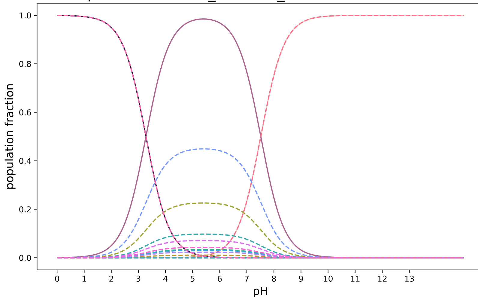
pKa-RobertRaddi_XGBoost_modified:SAMPL8-21
