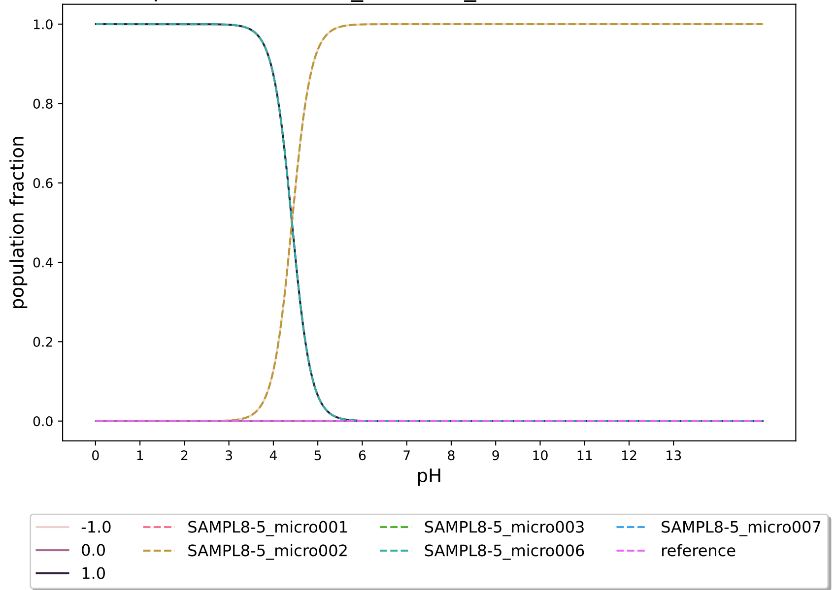
pKa-RobertRaddi_XGBoost_modified:SAMPL8-5
