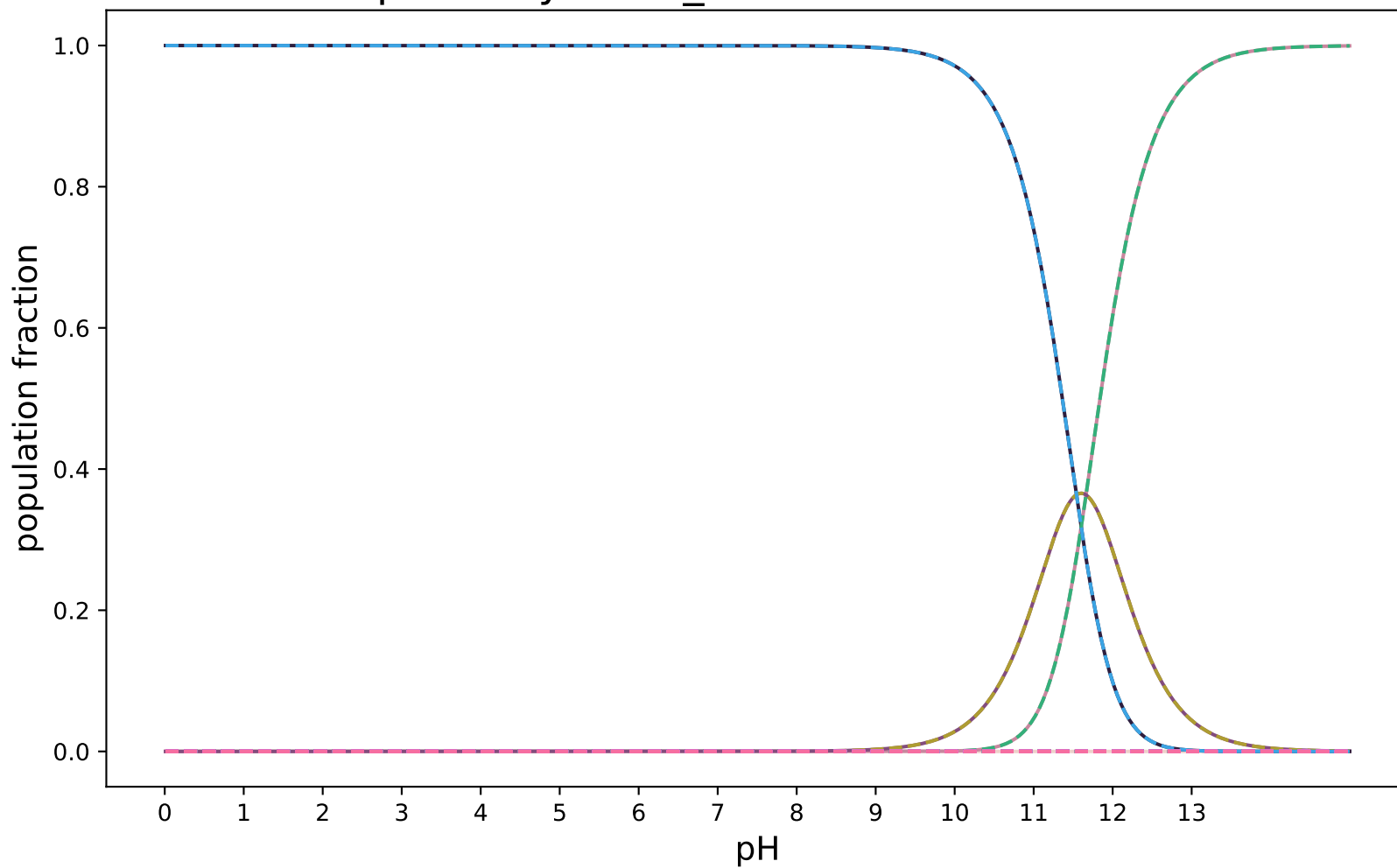
pKa-ZhiyiWu-1 modified:SAMPL8-14
