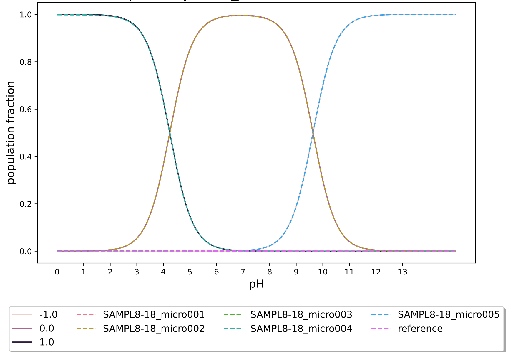
pKa-ZhiyiWu-1_modified:SAMPL8-18
