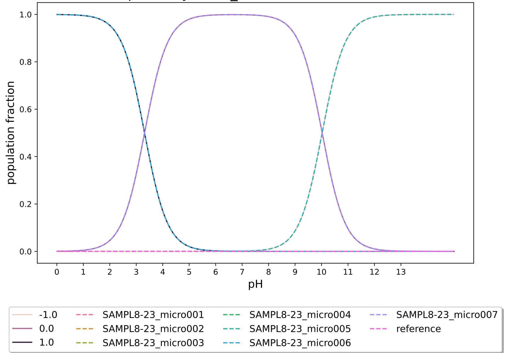
pKa-ZhiyiWu-1_modified:SAMPL8-23
