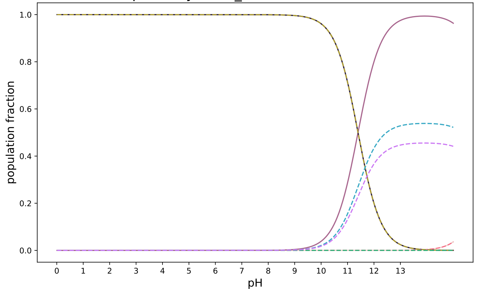
pKa-ZhiyiWu-1_modified:SAMPL8-7
