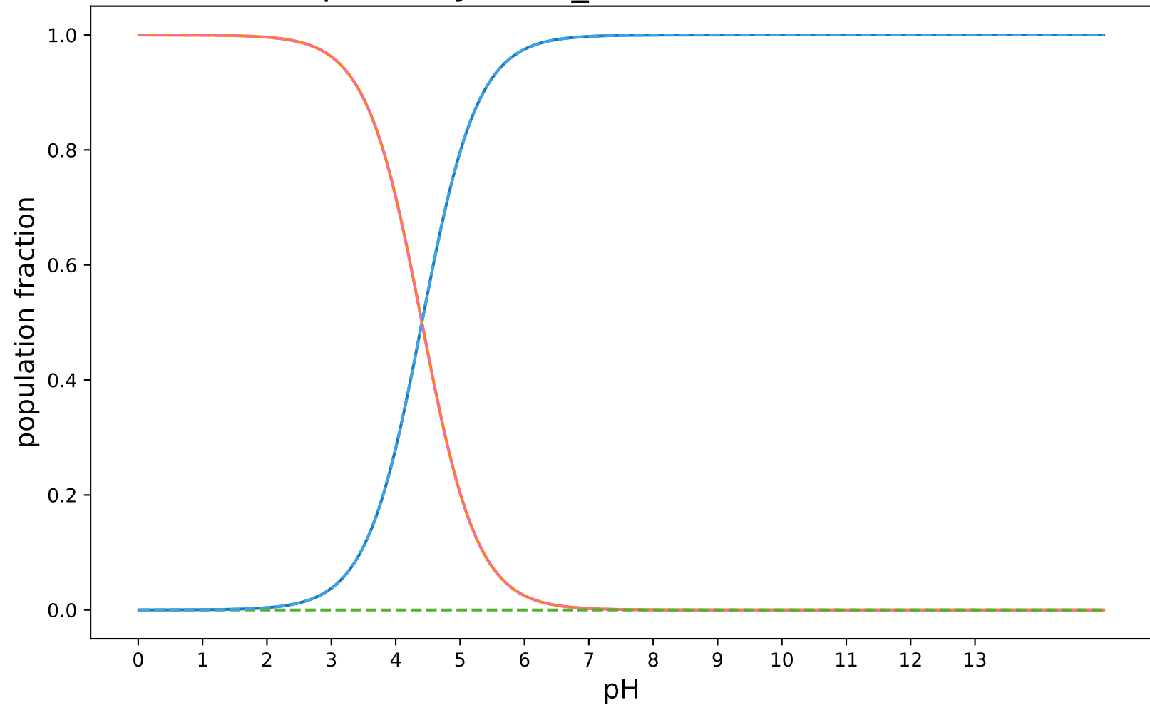
pKa-ZhiyiWu-1_modified:SAMPL8-8
