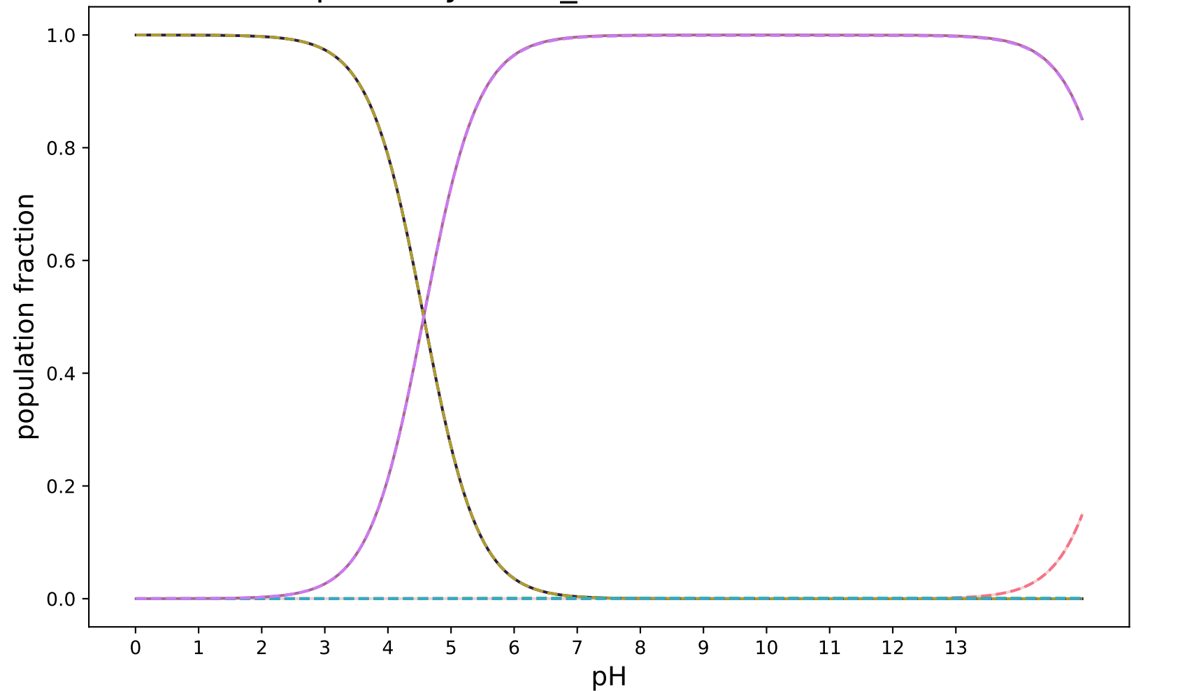
pKa-ZhiyiWu-1_modified:SAMPL8-9
