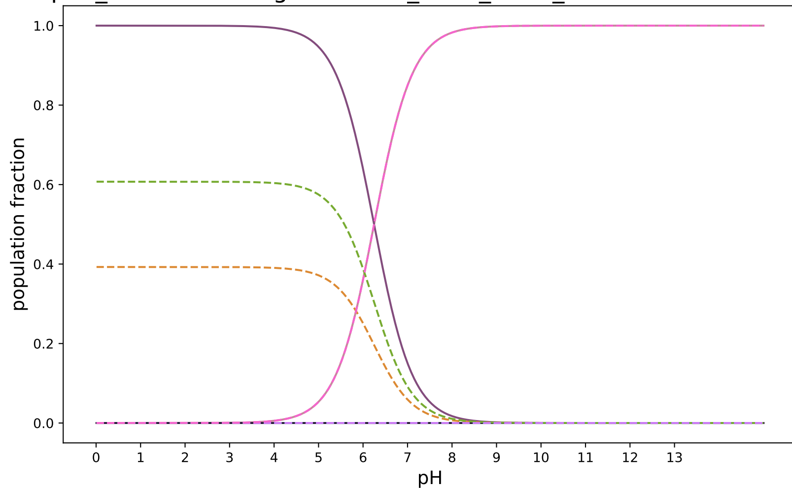
pKa_SabatinoRodriguezPaluch_uESE_extra_modified:SAMPL8-12
