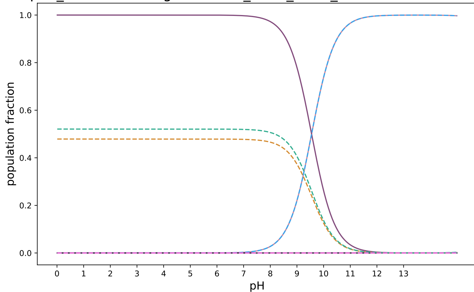
pKa_SabatinoRodriguezPaluch_uESE_extra_modified:SAMPL8-22
