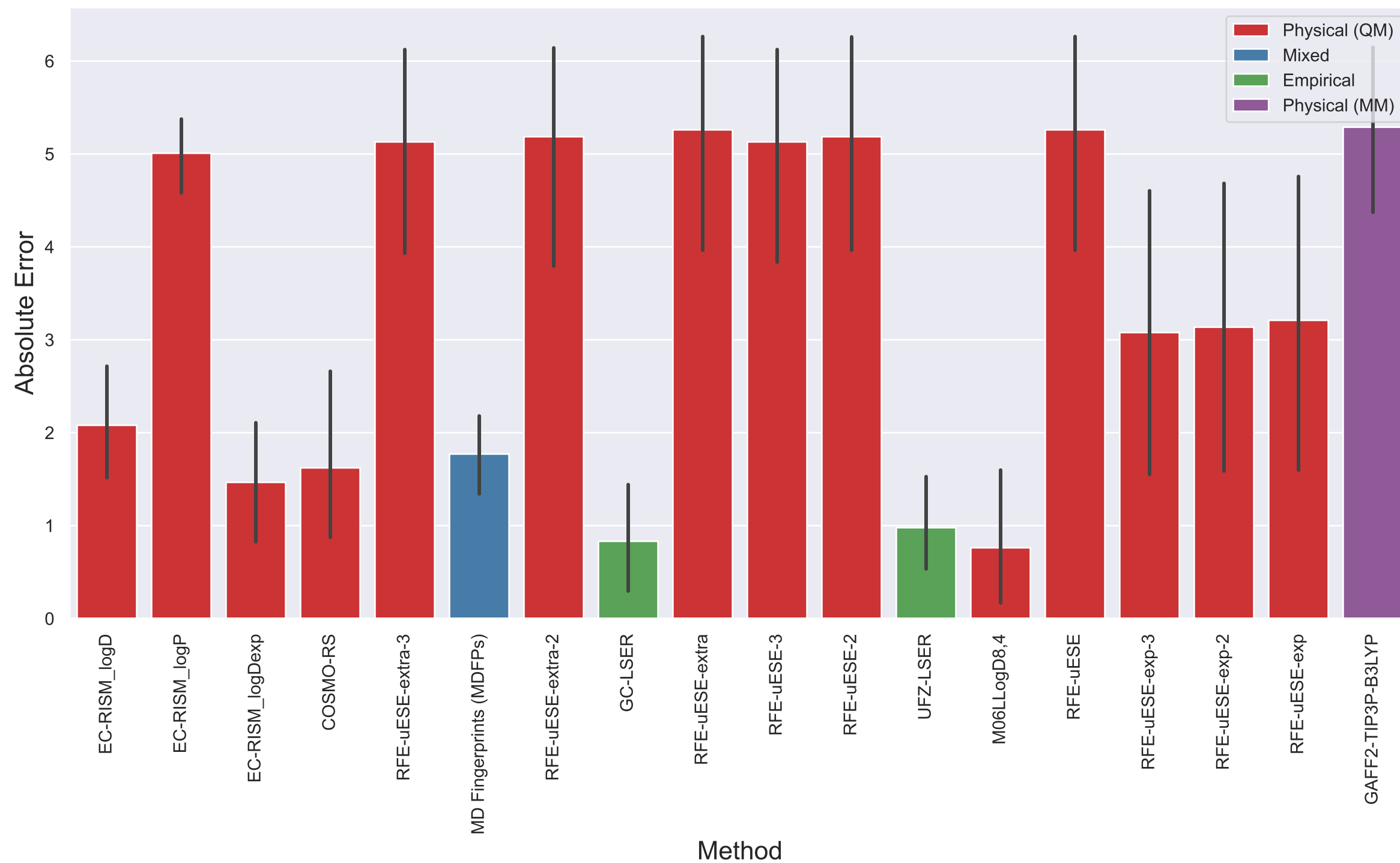
Absolute Error Plot for TBME-water
