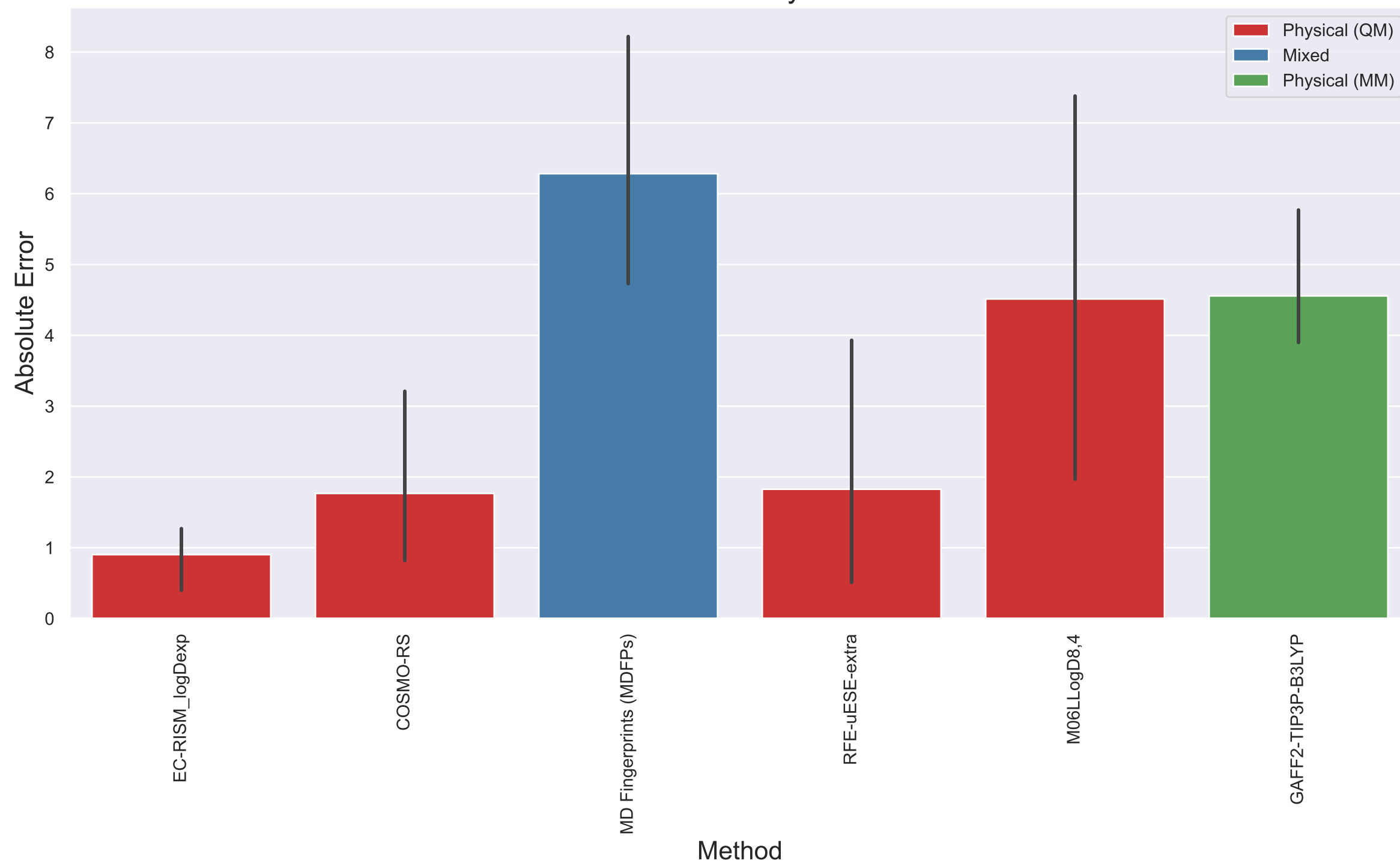
Absolute Error Plot for Cyclohexane-DMF
