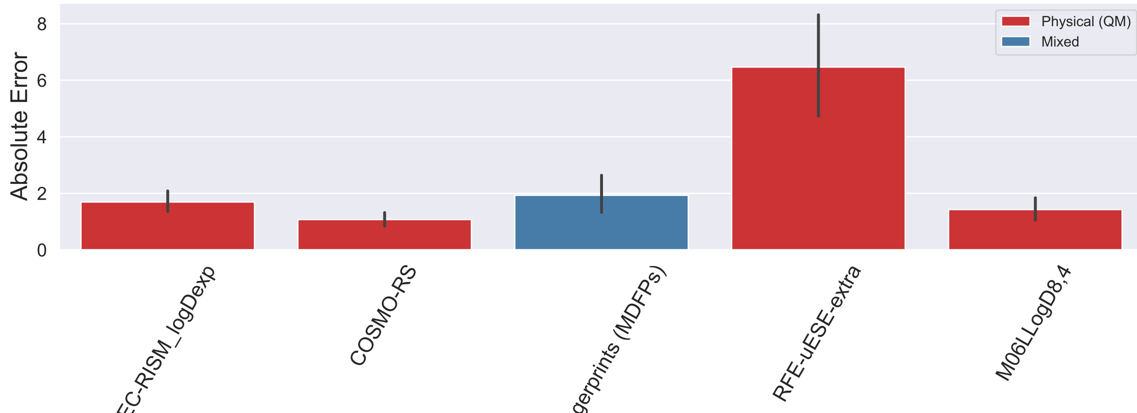
Absolute Error Plot Based on Method-All Solvent Combinations
