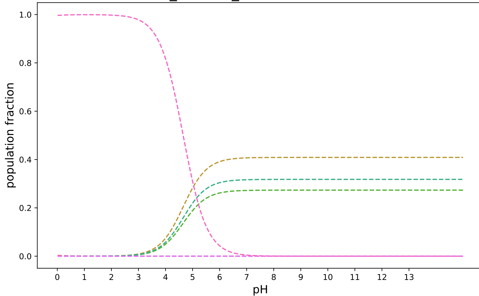
PKA_ECRISM_modified:SAMPL8-1
