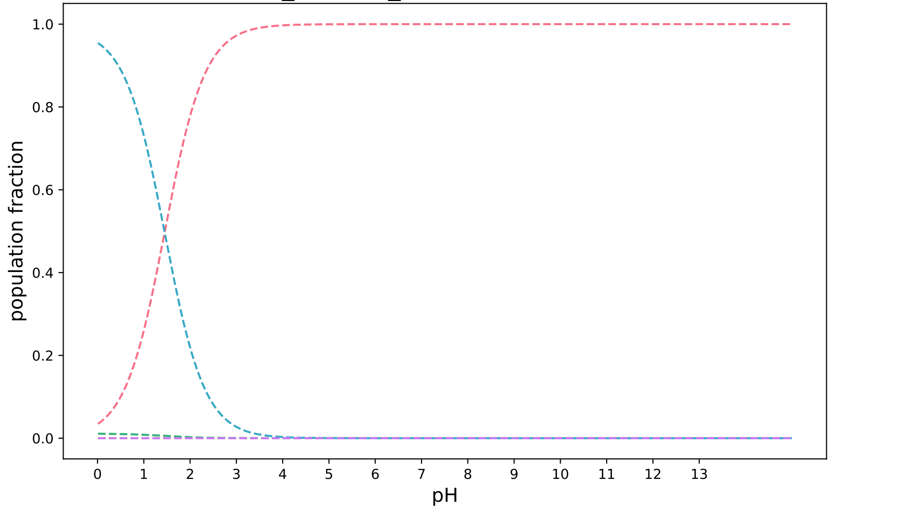
PKA_ECRISM_modified:SAMPL8-15
