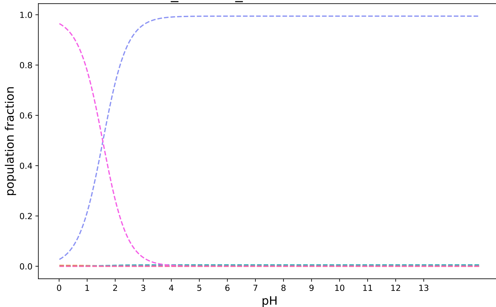
PKA_ECRISM_modified:SAMPL8-20
