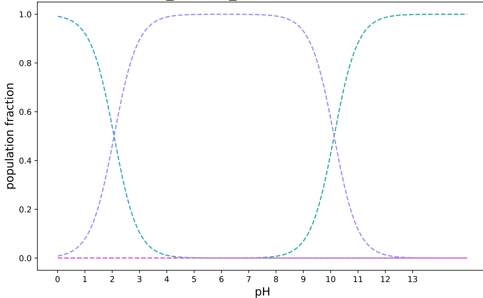
PKA_ECRISM_modified:SAMPL8-23
