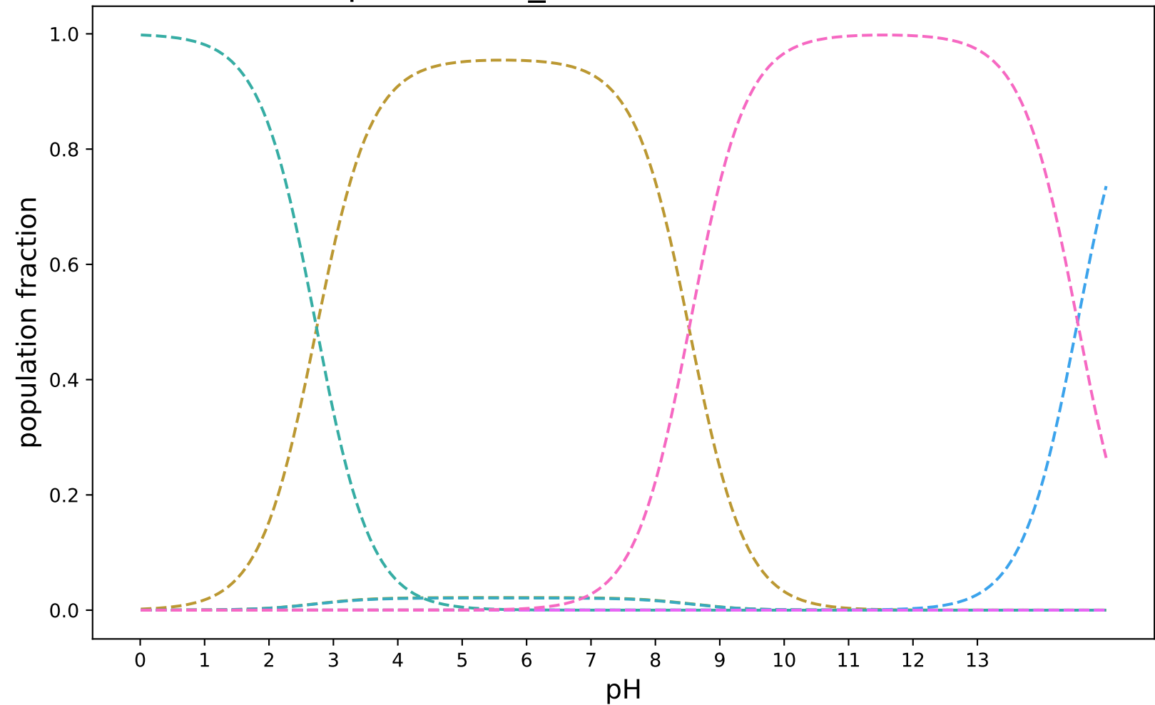
pKa-3DS-1_modified:SAMPL8-12
