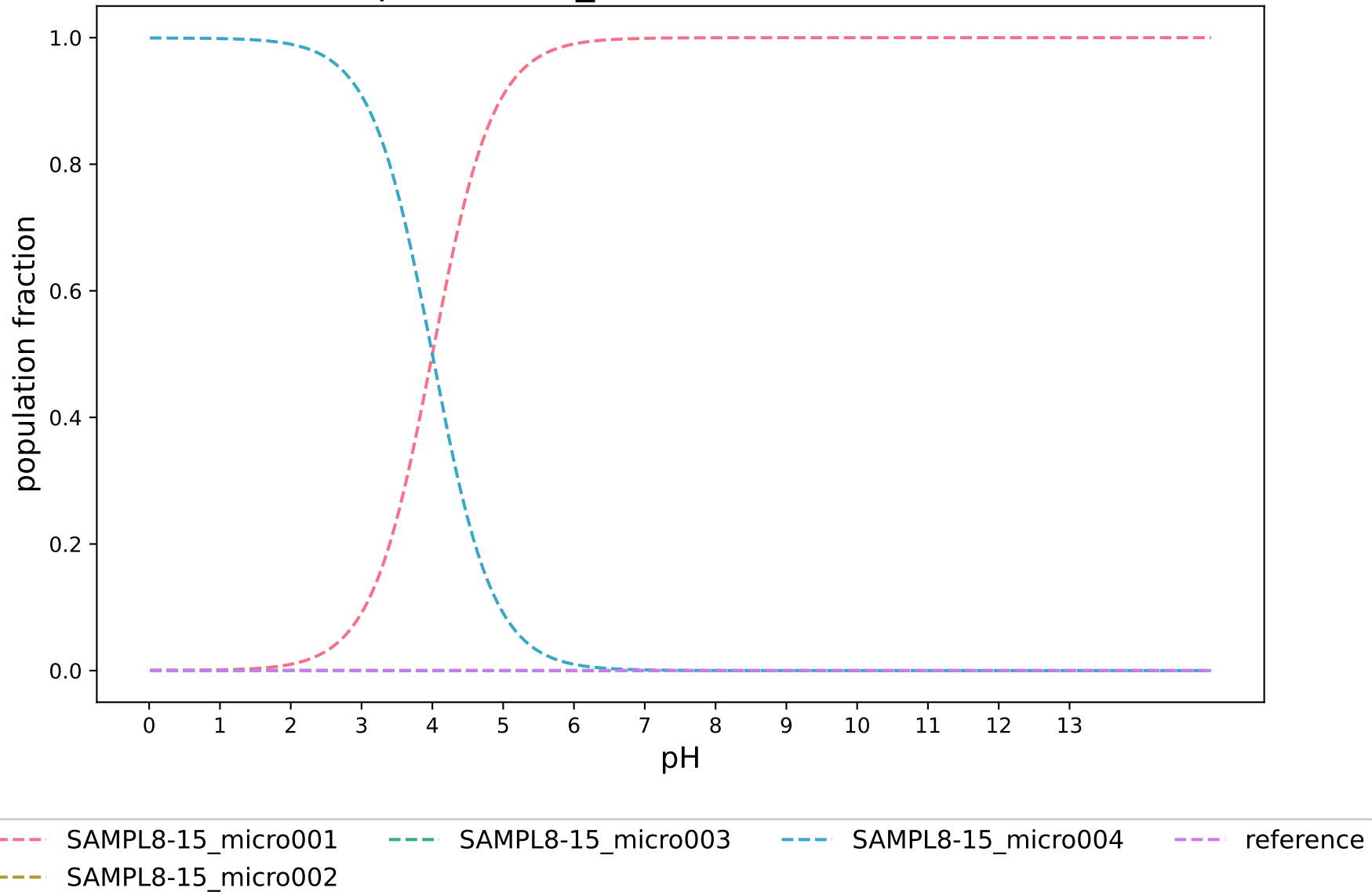
pKa-3DS-1_modified:SAMPL8-15
