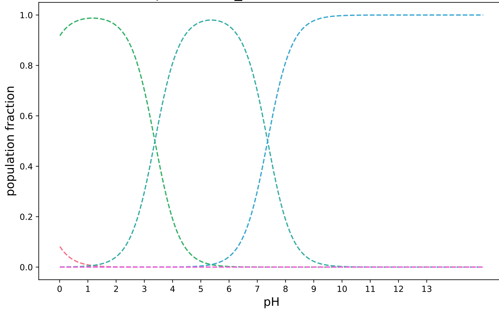
pKa-3DS-1_modified:SAMPL8-3
