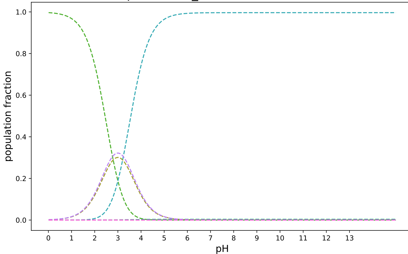
pKa-3DS-1_modified:SAMPL8-4
