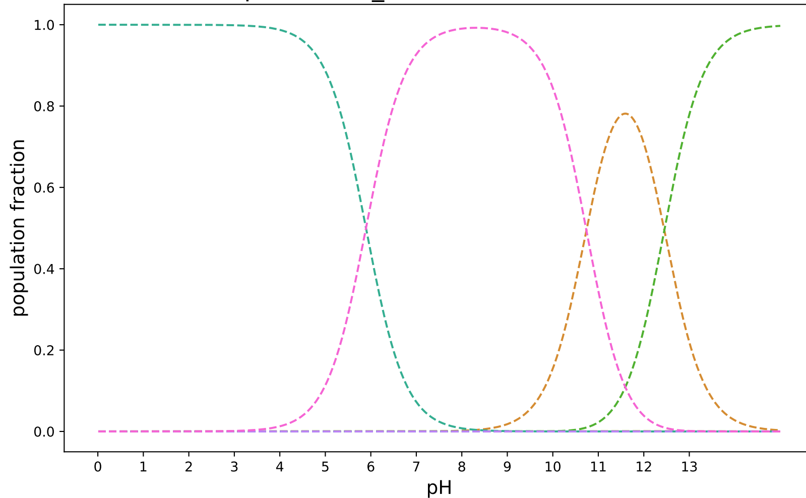
pKa-3DS-2_modified:SAMPL8-16
