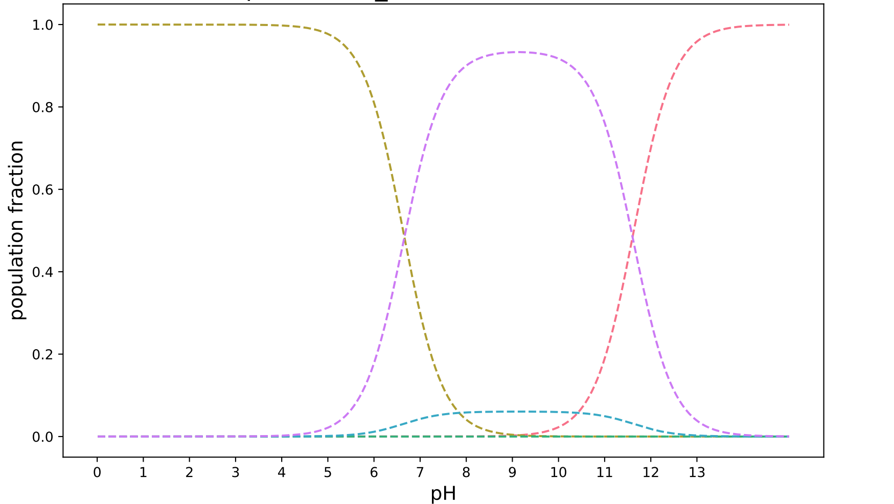
pKa-3DS-2_modified:SAMPL8-17
