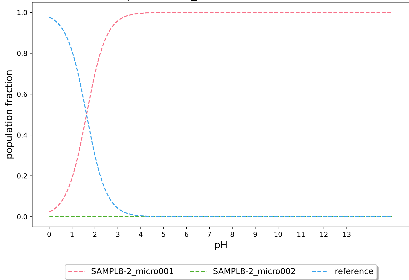
pKa-3DS-2_modified:SAMPL8-2
