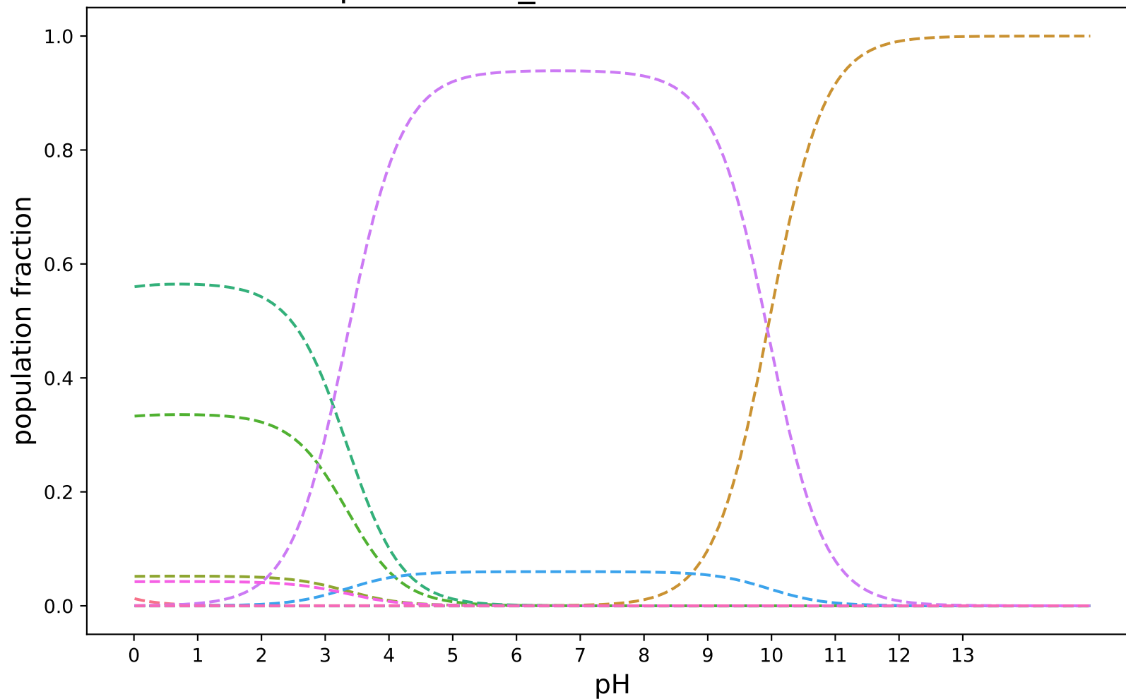
pKa-3DS-2_modified:SAMPL8-20
