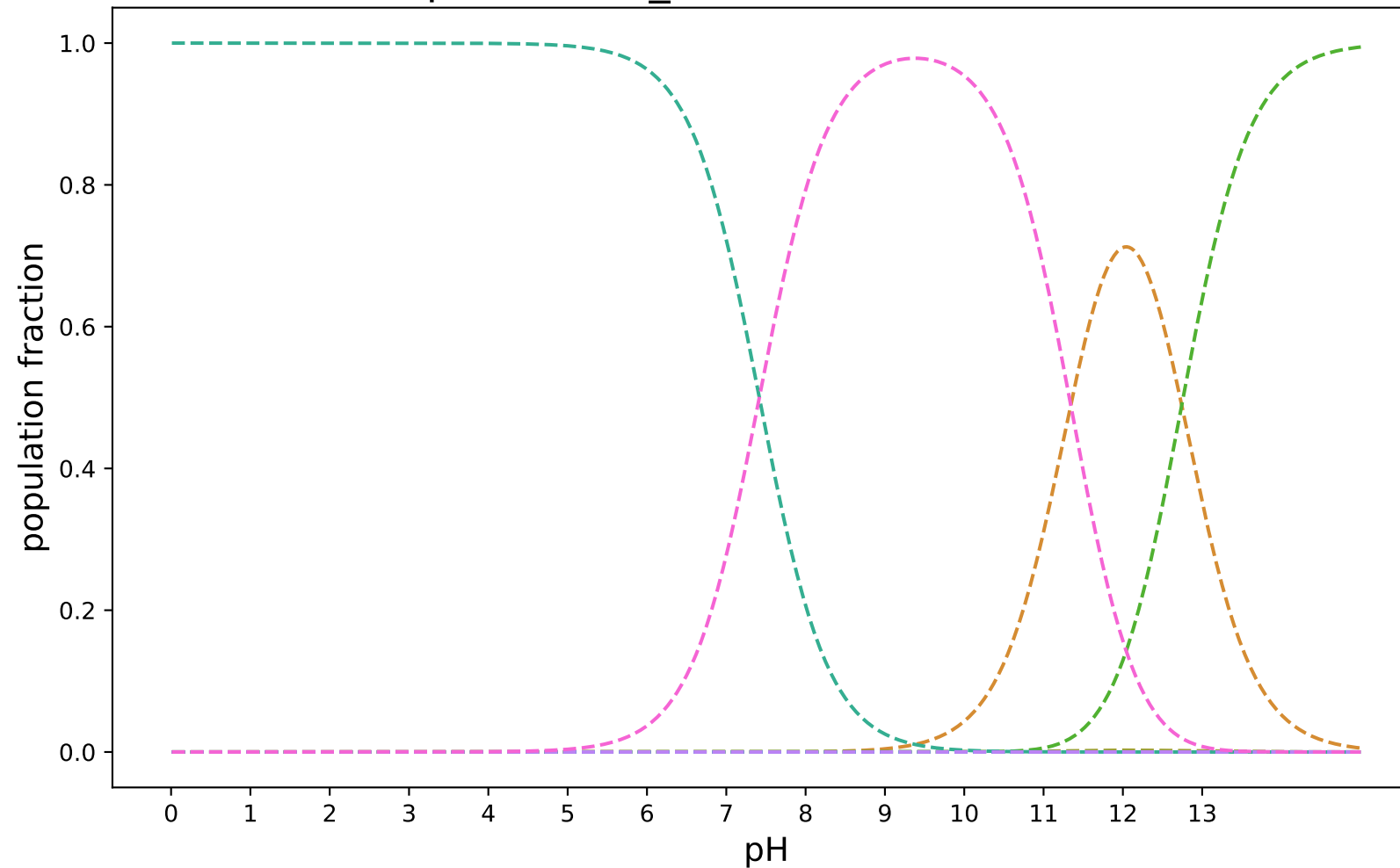
pKa-3DS-3_modified:SAMPL8-16
