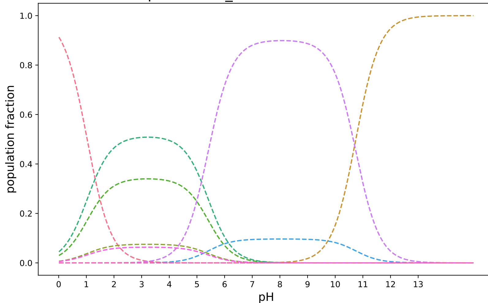
pKa-3DS-3_modified:SAMPL8-20
