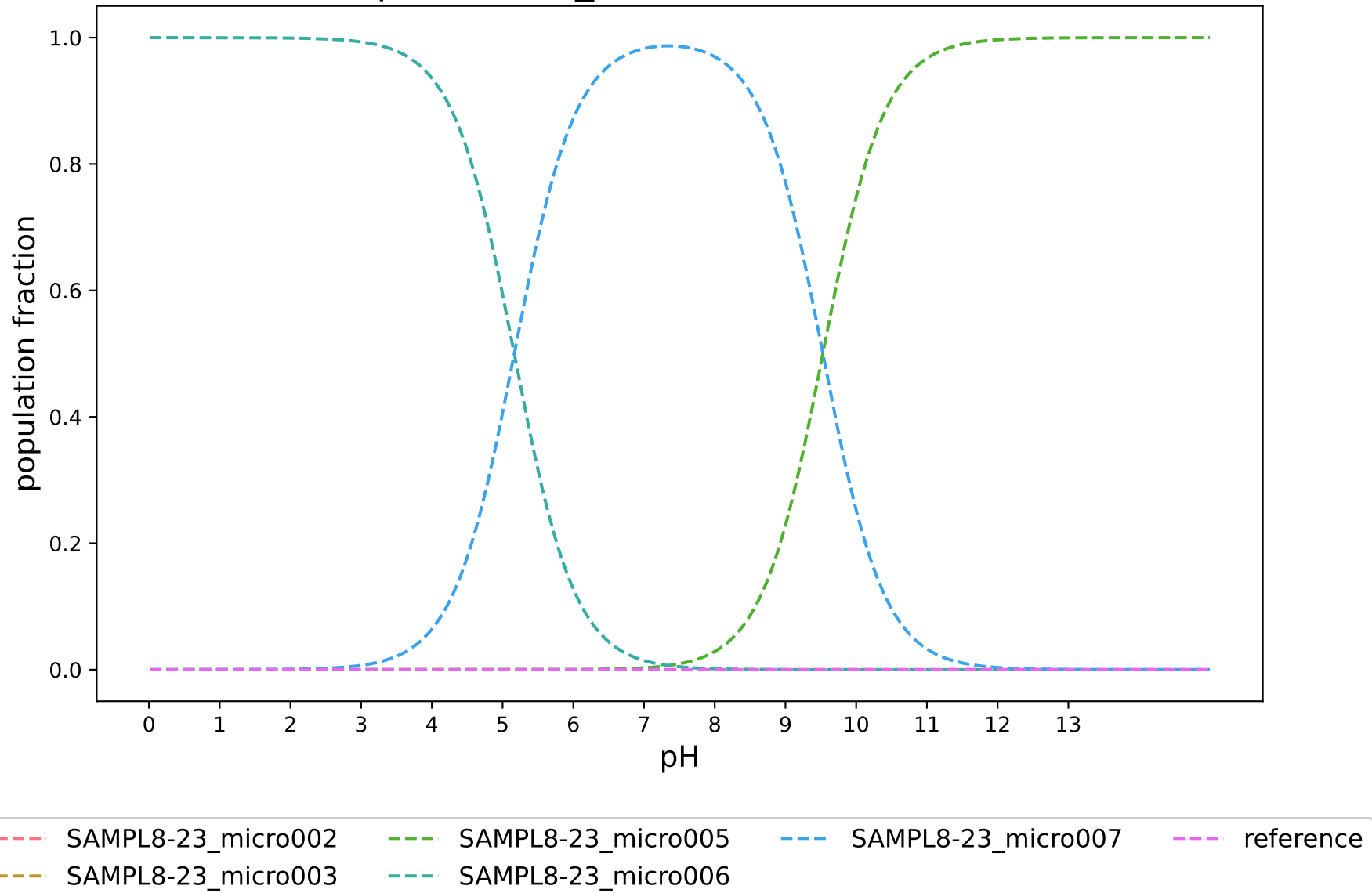
pKa-3DS-3_modified:SAMPL8-23
