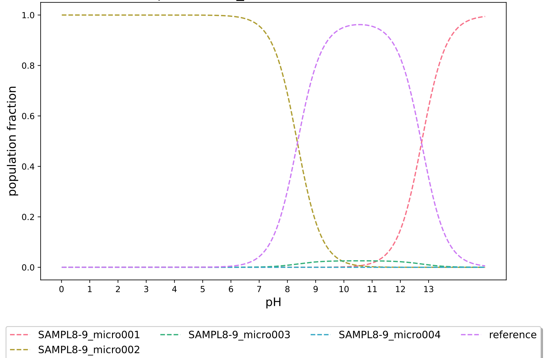
pKa-3DS-3_modified:SAMPL8-9
