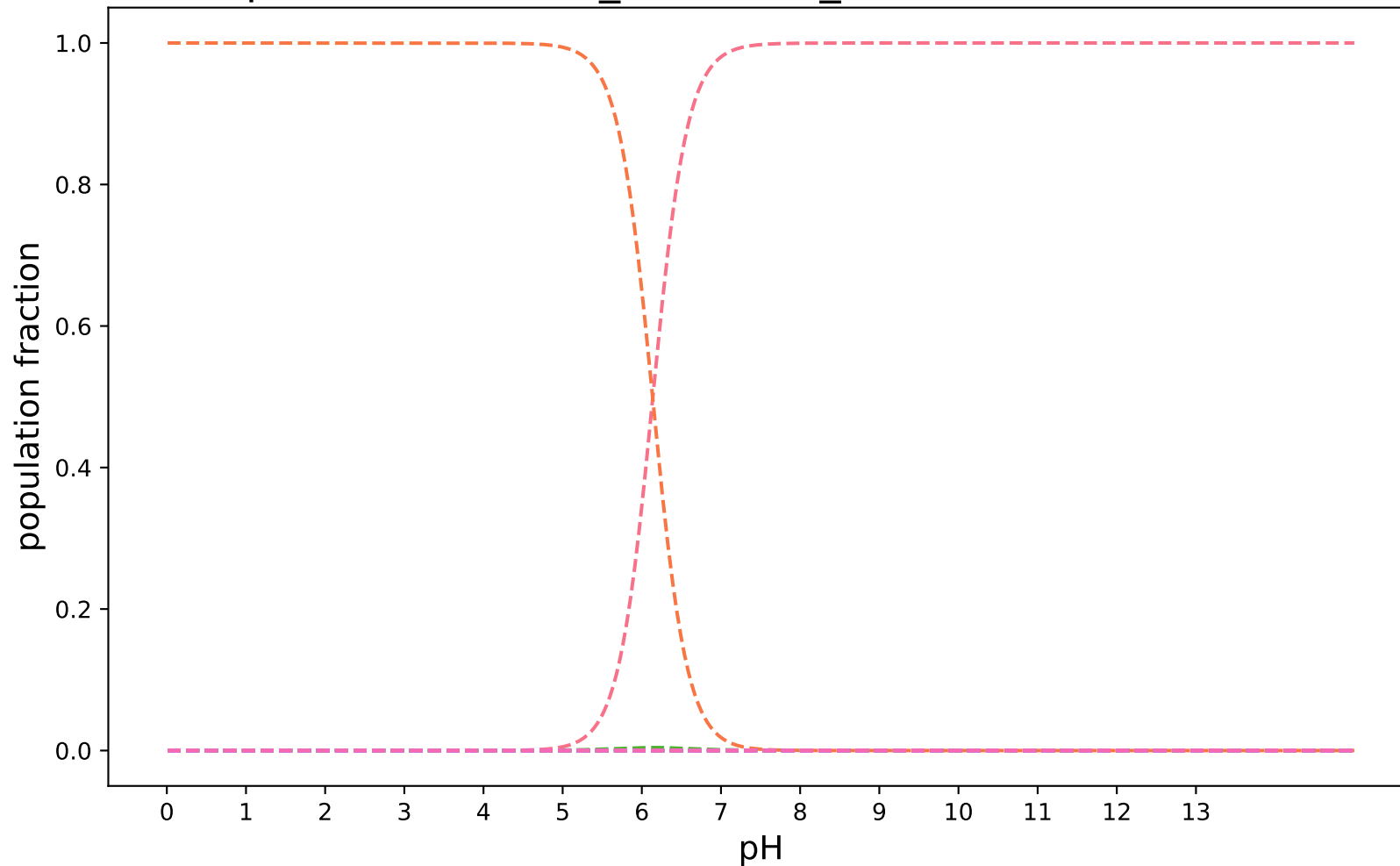
pKa-RobertRaddi_AdaBoost_modified:SAMPL8-14
