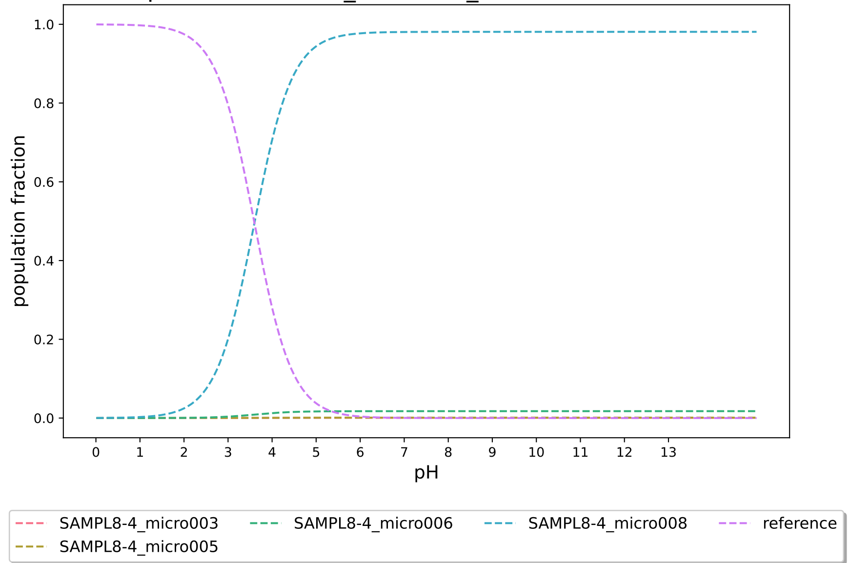
pKa-RobertRaddi_AdaBoost_modified:SAMPL8-4
