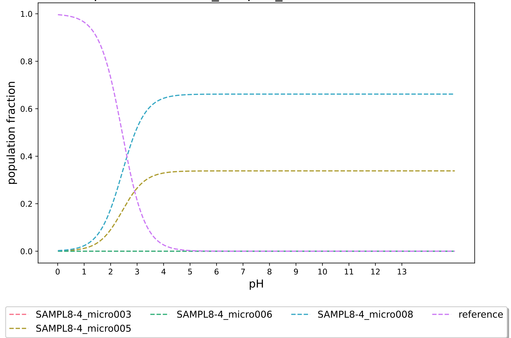
pKa-RobertRaddi_DeepGP_modified:SAMPL8-4
