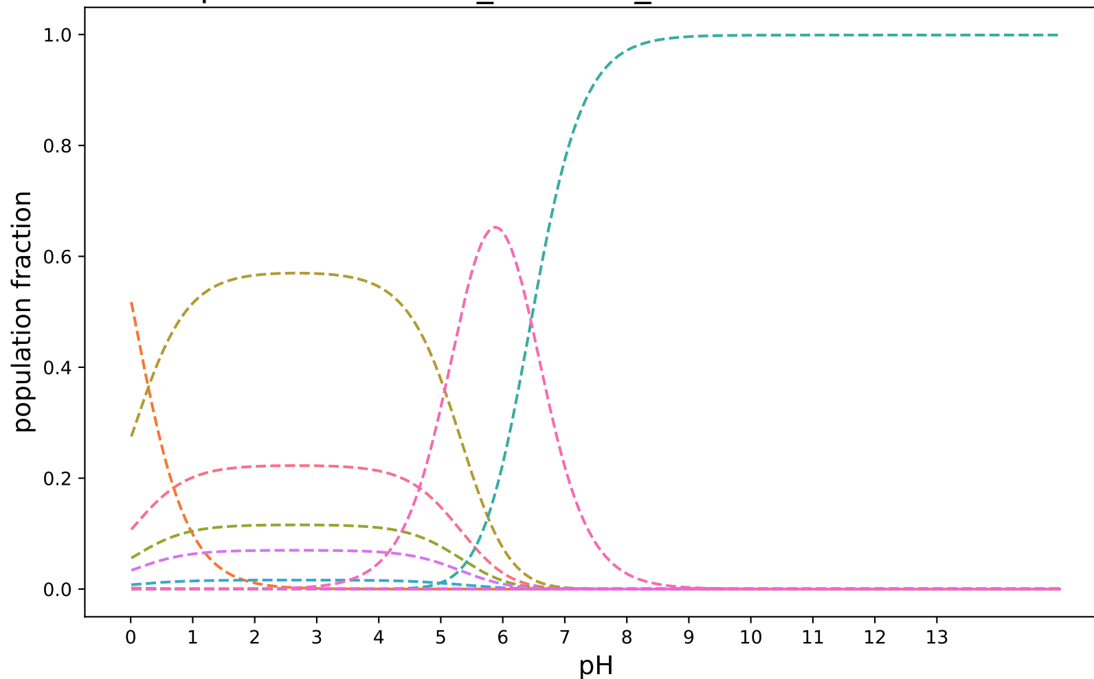
pKa-RobertRaddi_XGBoost_modified:SAMPL8-19
