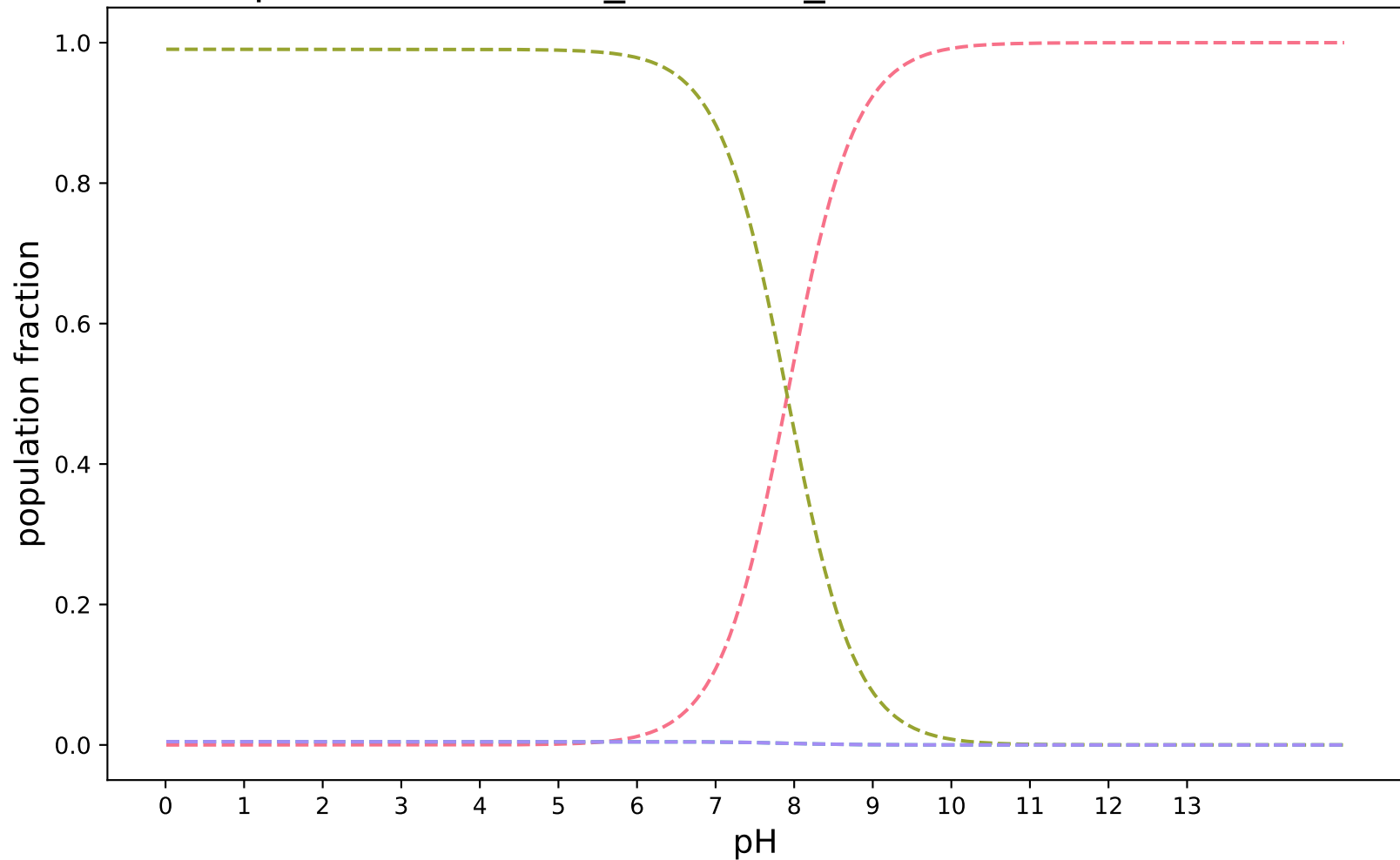
pKa-RobertRaddi_XGBoost_modified:SAMPL8-22
