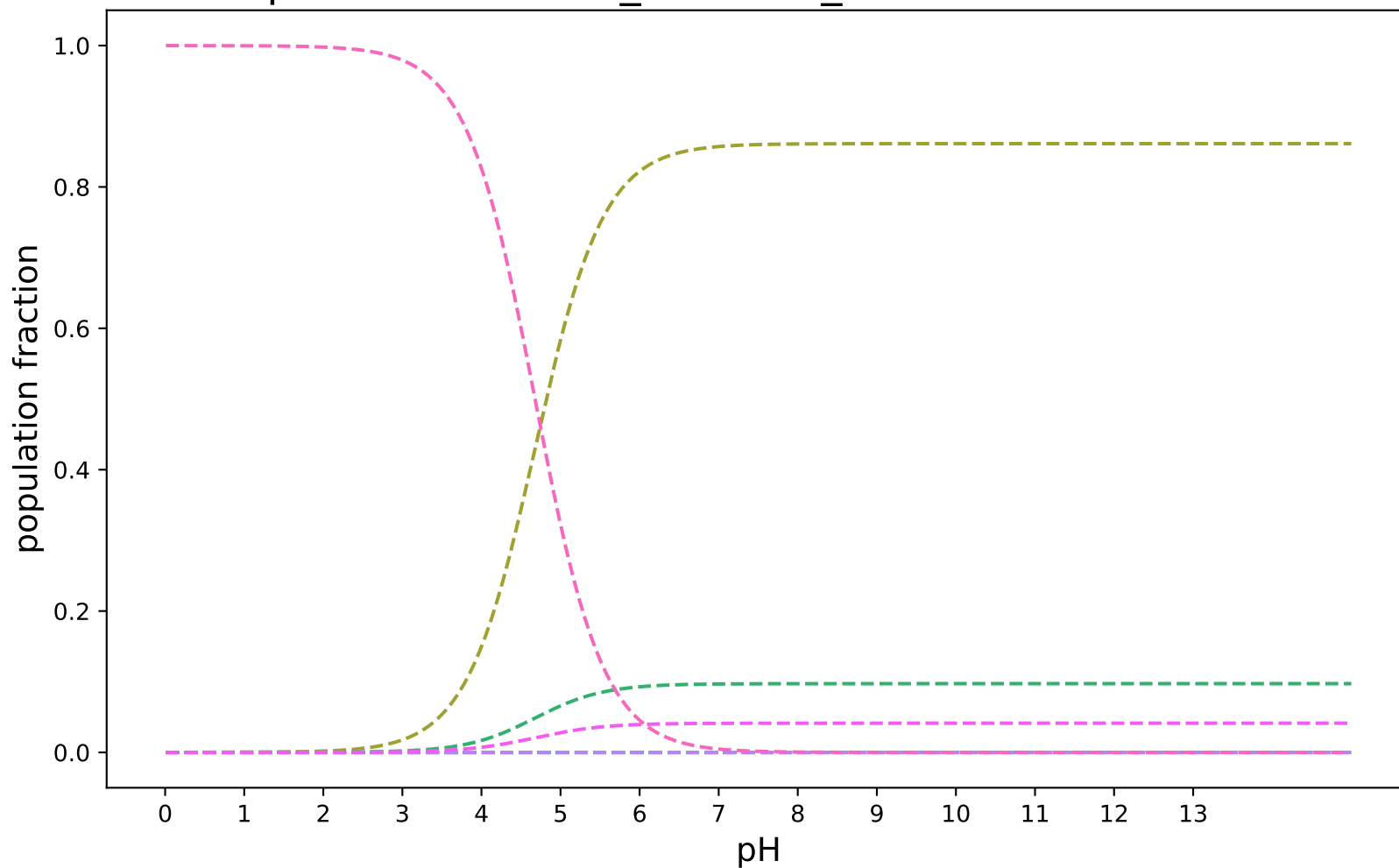
pKa-RobertRaddi_XGBoost_modified:SAMPL8-3
