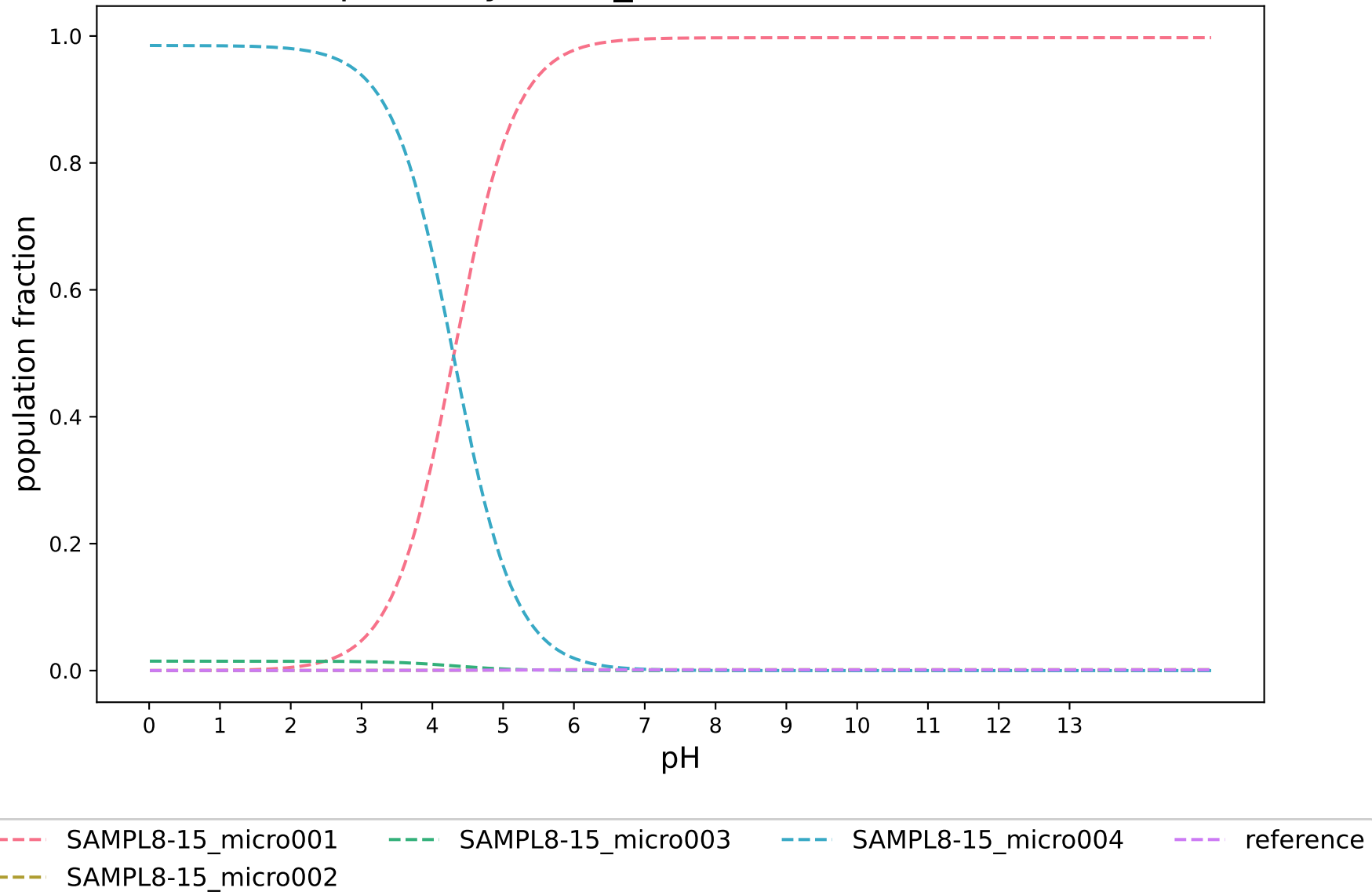
pKa-ZhiyiWu-1_modified:SAMPL8-15
