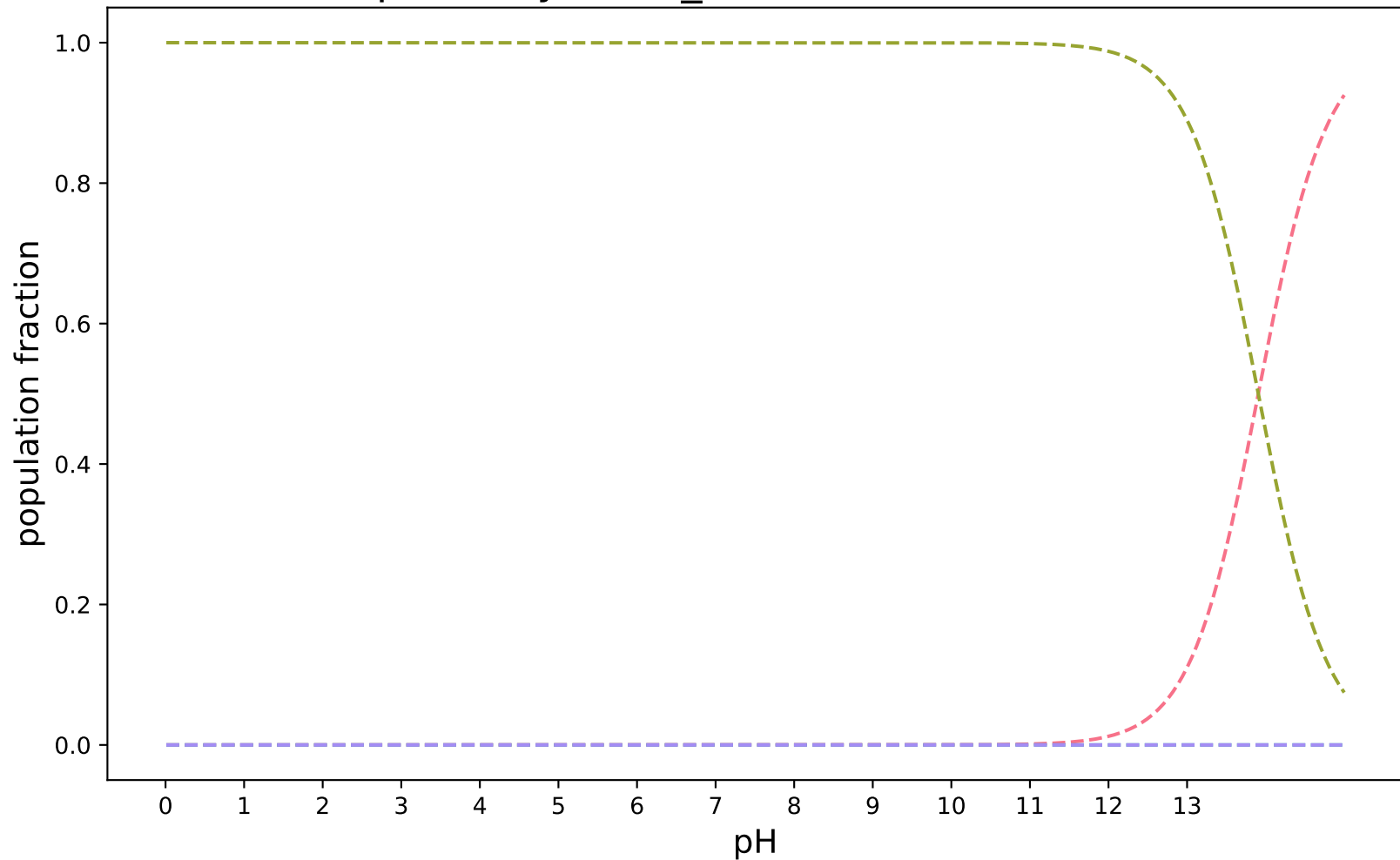
pKa-ZhiyiWu-1_modified:SAMPL8-22
