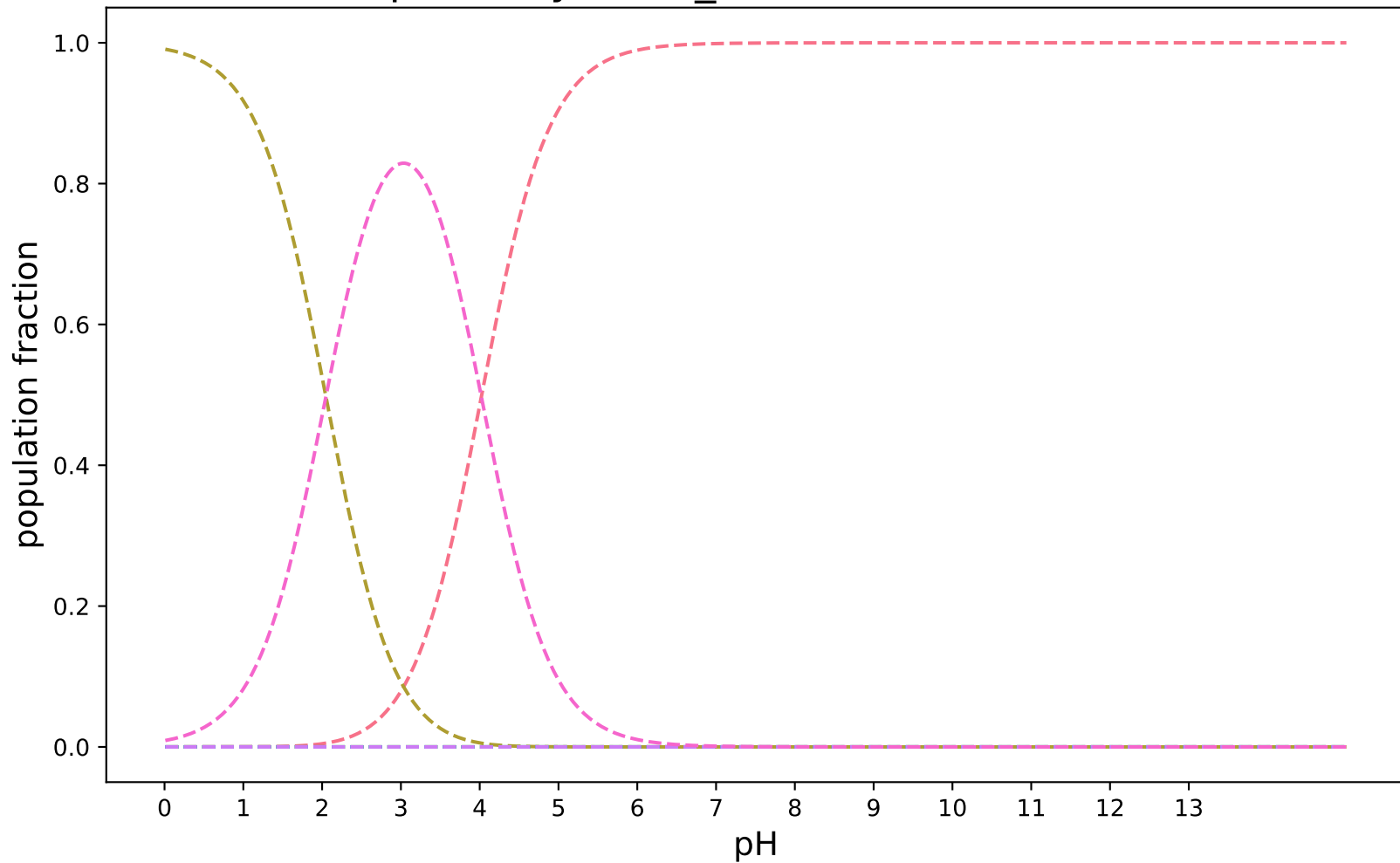
pKa-ZhiyiWu-1_modified:SAMPL8-6
