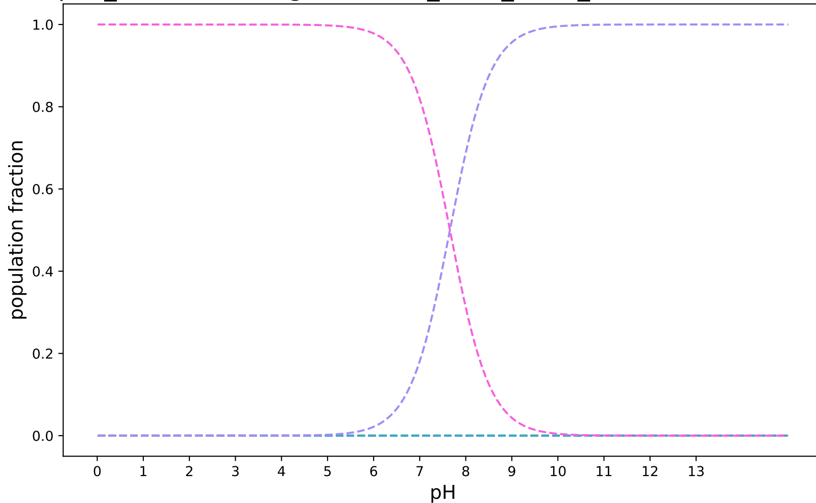
pKa_SabatinoRodriguezPaluch_uESE_extra_modified:SAMPL8-5
