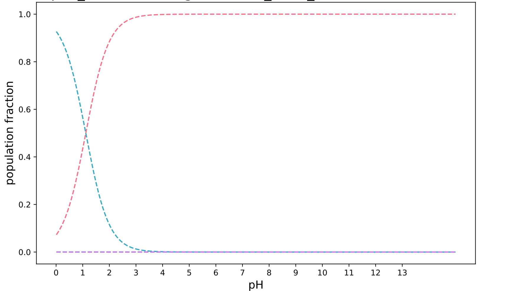
pKa_SabatinoRodriguezPaluch_uESE_modified:SAMPL8-15
