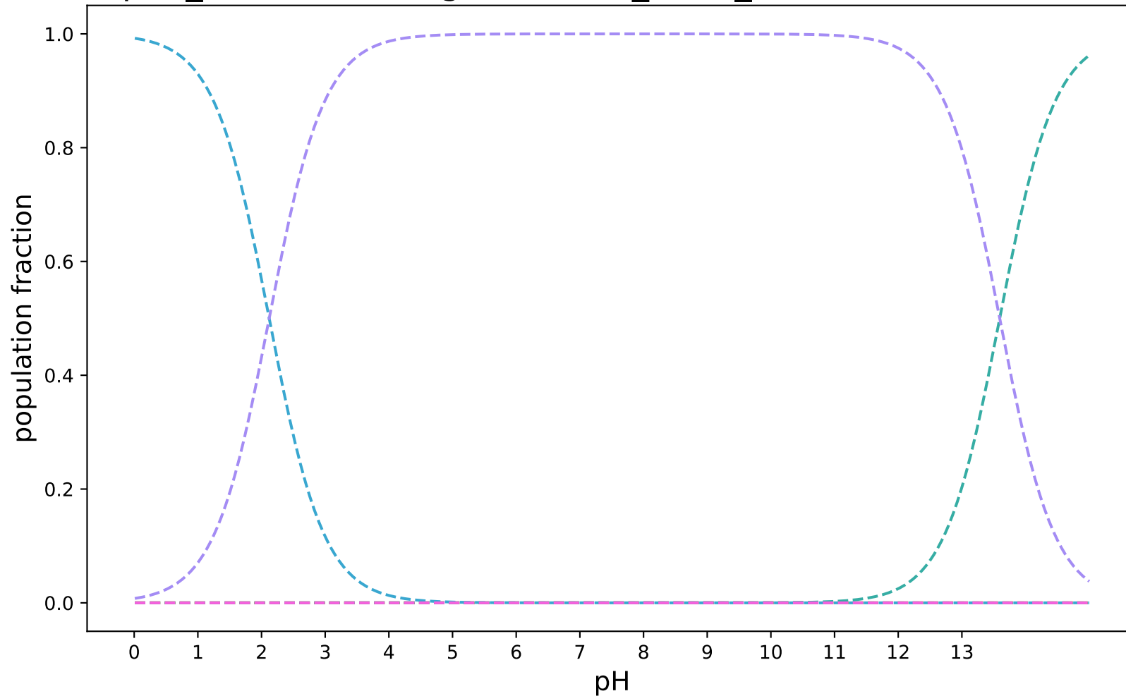
pKa_SabatinoRodriguezPaluch_uESE_modified:SAMPL8-23
